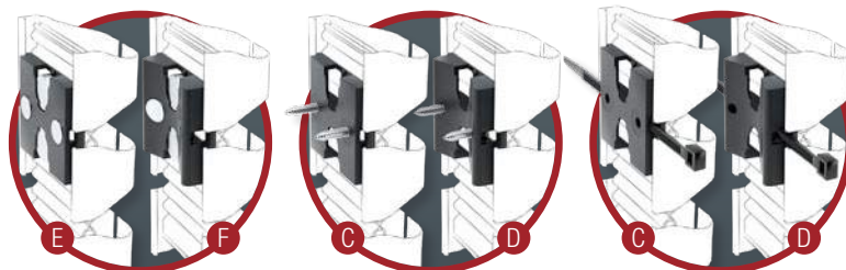
Connection C/E – for flat frames and Connection D/F – for round frames for mounting on the table frame (rectangular/ \varnothing = 70 mm) using integrated magnets E F , screws C D or cable ties C D
