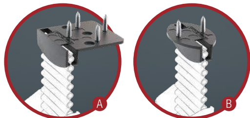
Connection A/B – angled/oval for table top for mounting underneath the table top or on the cable duct
